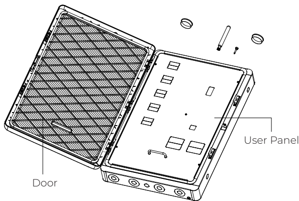
Fig. 3-1 ATI smart distribution panel
