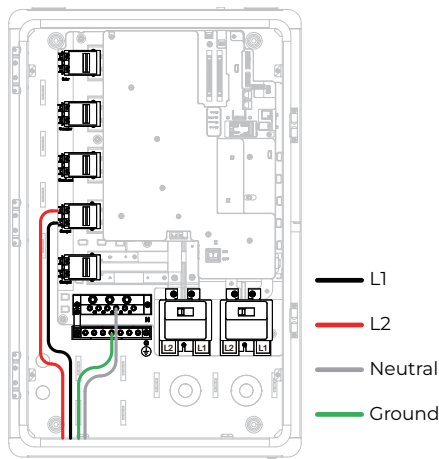
Fig. 7-14 Connecting to ESS1
