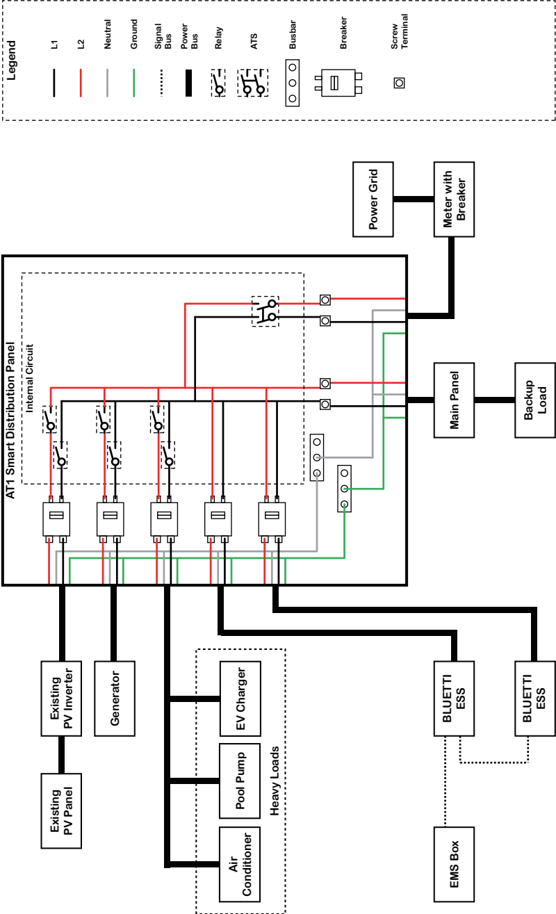
Fig. 7-21 Whole-home backup
