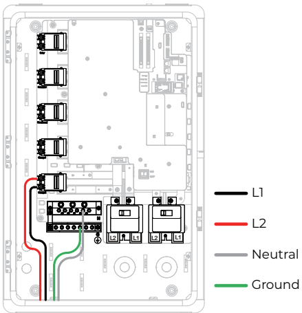
Fig. 7-15 Connecting to ESS2
