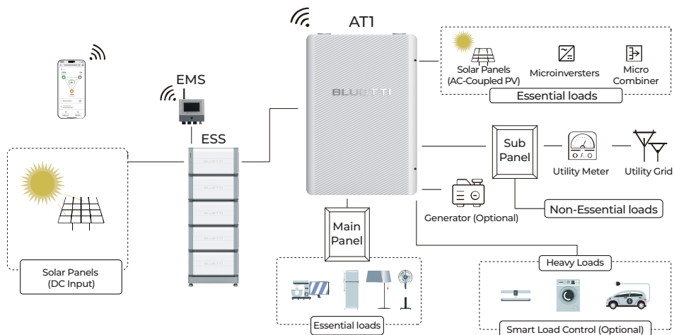
Fig. 7-2 Partial backup
